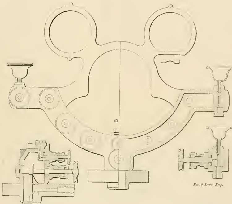
BOILER HEAD STAND.
